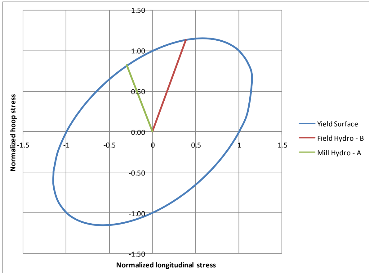
Figure A.1 von Mises Equation Represented as a Yield Ellipse
